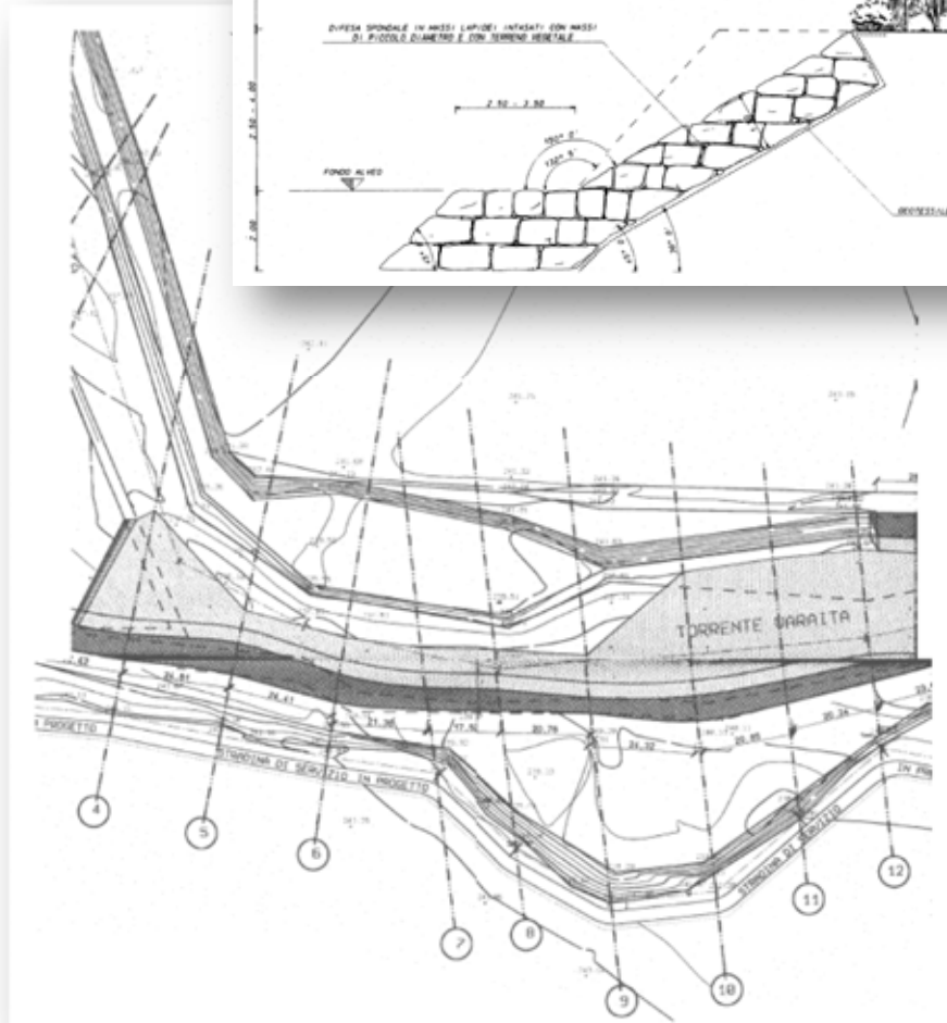
Plan of the protection of the embankment in the Type A project.
